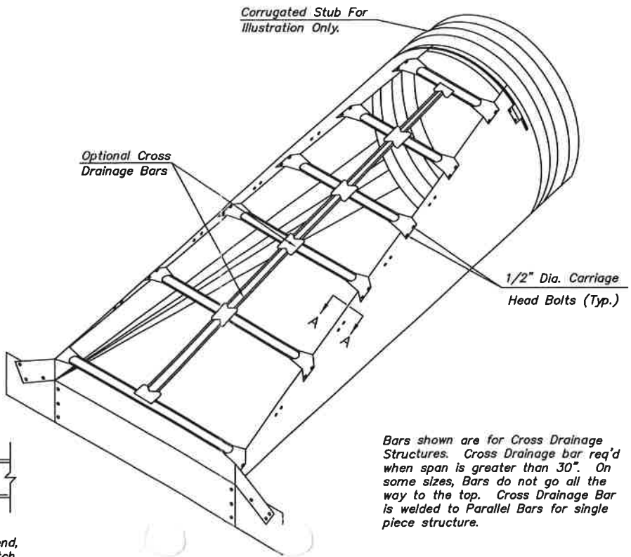
48" CROSS DRAINAGE STRUCTURE 6:1 SLOPE
