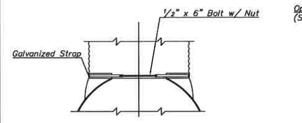
TYPE #1 CONNECTOR DETAIL
