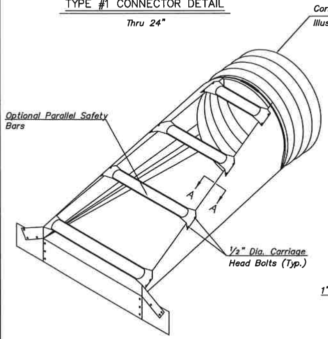
24" PARALLEL DRAINAGE STRUCTURE 6:1 SLOPE
