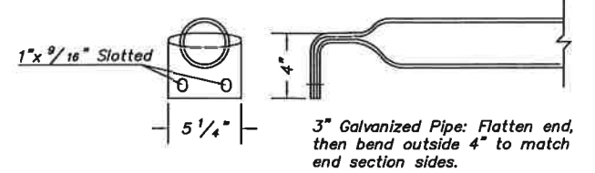
PARALLEL BARS DETAIL OF OPTIONAL SAFETY BARS
